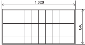
(CS-260B61S 外形図)
