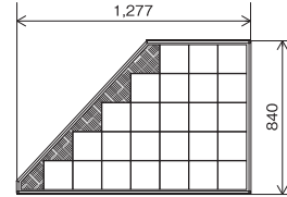
(CS-124B61L 外形図)
