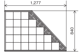
(CS-124B61R 外形図)
